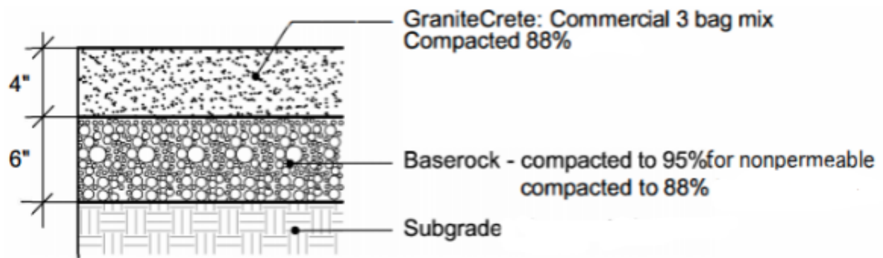
GraniteCrete Paving - EVA & Vehicular Traffic
